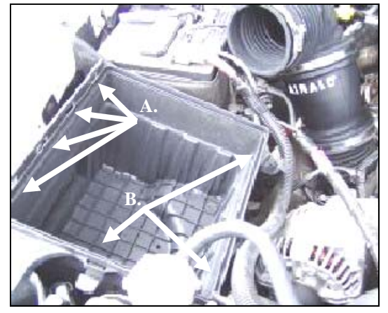
12. A.) Install the CAD by inserting the four tabs into the side of the factory airbox. B.) Relatch the three airbox clips onto the CAD.
