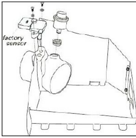
11. Install the factory MAF sensor into the air filter adapter using two 8-32 button head screws (#12), and #8 flat washers (#13). Install the factory rubber grommet and filter minder into the air filter adapter.
