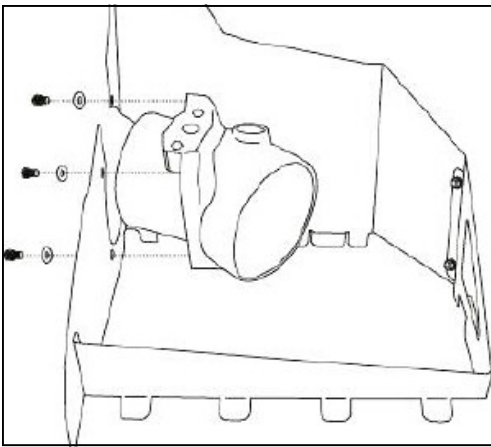
10. Mount the air filter adapter (#5) onto the CAD, using three 1/4-20x 5/8" hex bolts (#10), and three 1/4" flat washers (#11).
