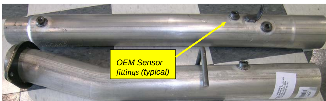
Ford 6.4L replacement pipe set (example is a 'delete' pipe manufactured by Flow-Pro)
