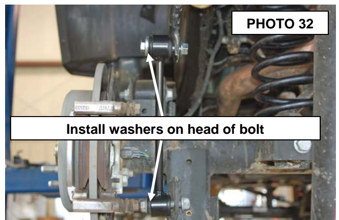
Bolt shown pointed toward rear of vehicle
